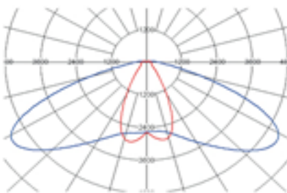
Luminance Intensity Distribution
